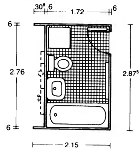
⑩ Bathroom cubicle with washing machine
